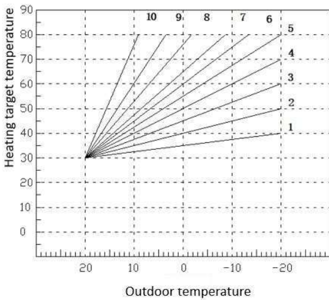
Compensation curve (offset =30)
