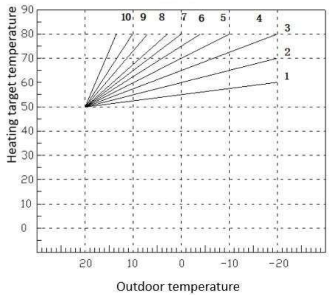
Compensation curve (offset =50)
