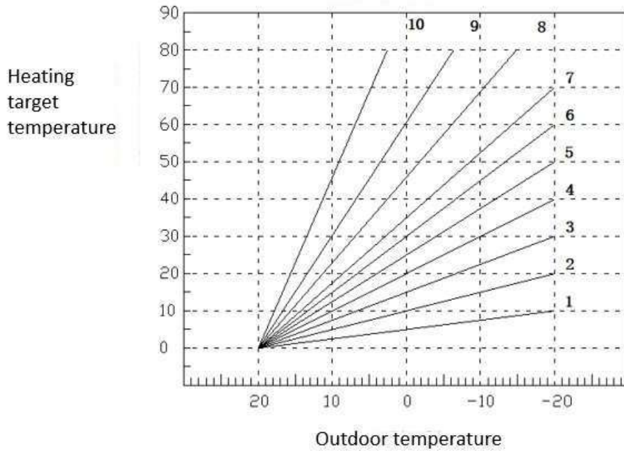
Compensation curve (offset =0)
